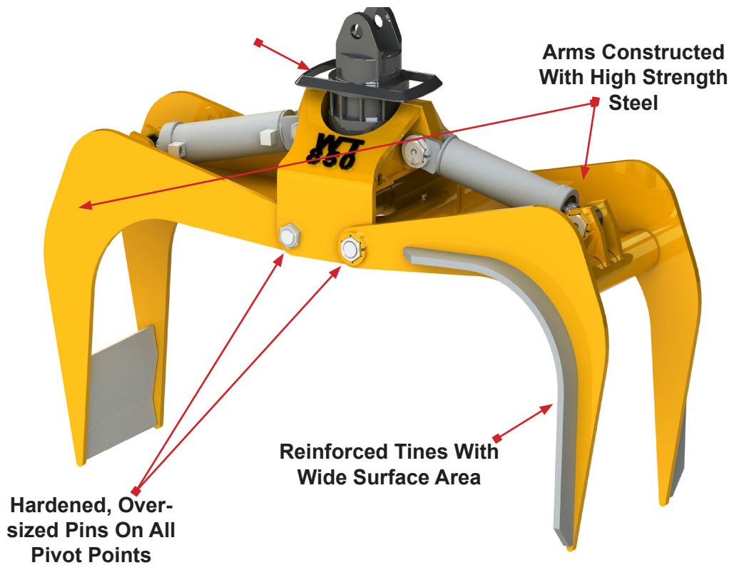
Heavy Duty Rotator (20" Bearing)
